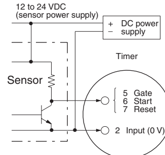
Operates with transistor ON
