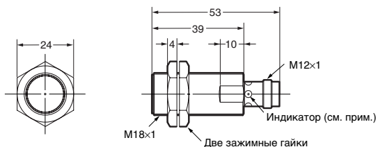
E2A-M18KS08-M1-□□/E2A-S18KS08-M1-□
